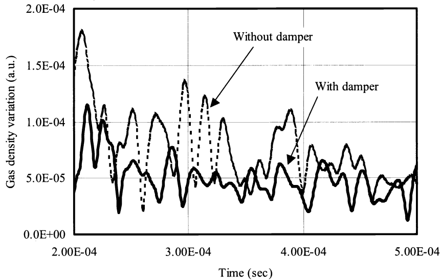
Fig. 1 Calculated gas density variation in the discharge region with and without acoustic wave damper.
