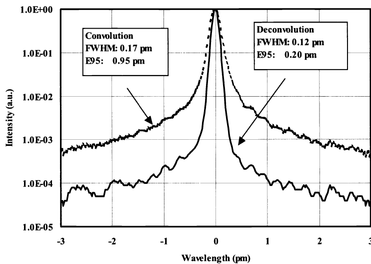
Fig. 3 Spectra for the whole laser beams measured by a HEXA spectrometer
