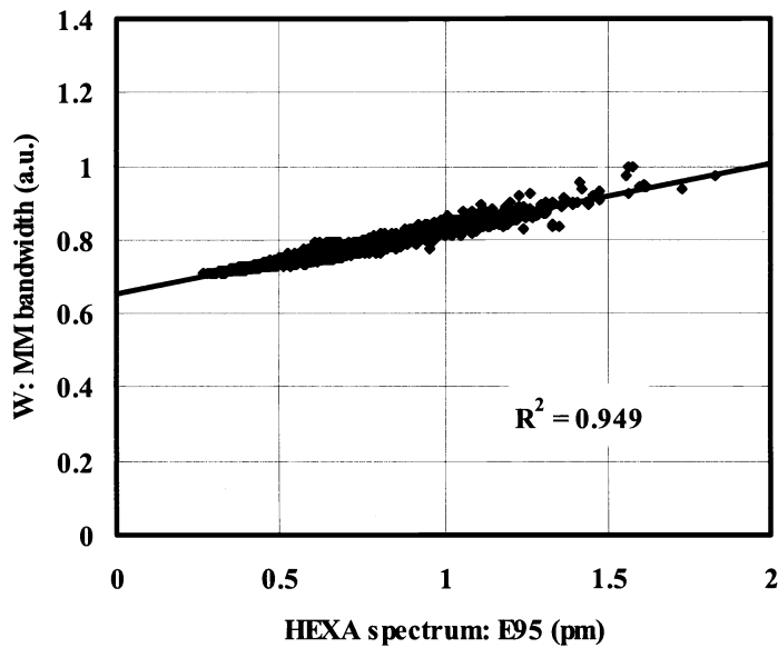
Fig. 2 The relationship between HEXA E95 and MM bandwidth.
