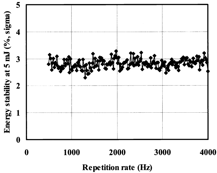
Fig. 7 Energy stability (sigma) as a function of repetition rate
