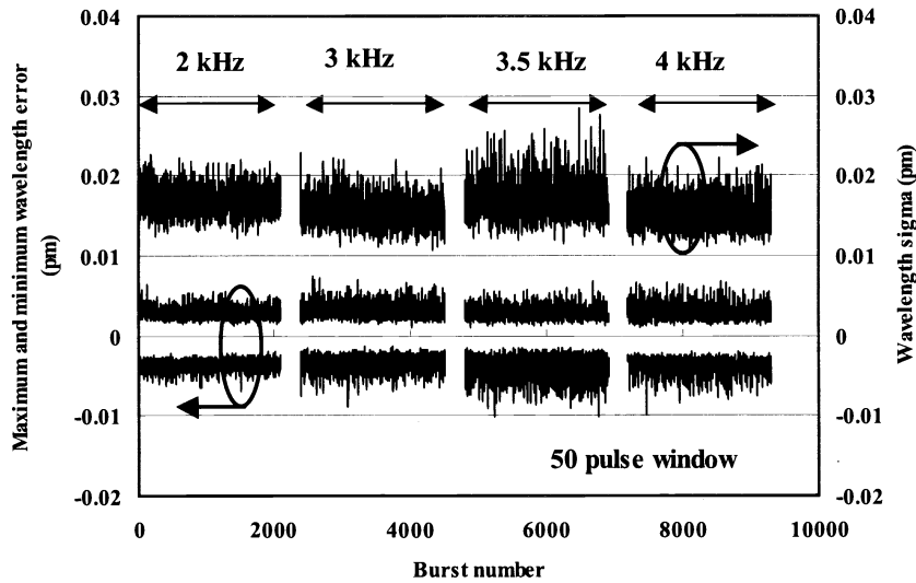
Fig. 6 Average wavelength stability and wavelength stability sigma in middle term operation (50 pulse window)
