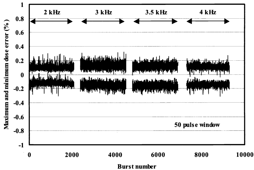
Fig. 8 Energy dose stability in middle term operation
