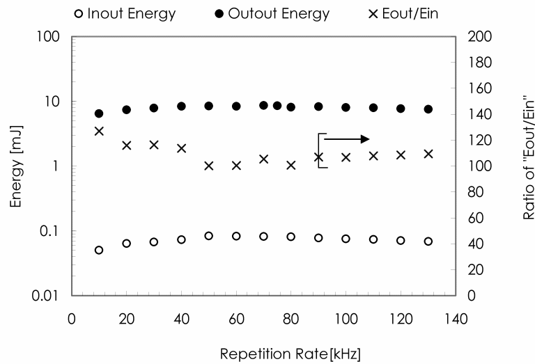
Figure.5 Dependence of amplified pulse energies on the repetition rate of the laser system
