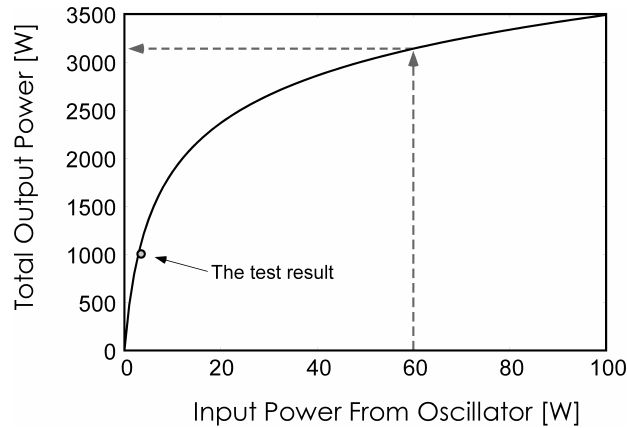
Figure.3 Output power estimation of the RF-excited MOPA system by use of a short pulse 60 W input power from an oscillator. The amplification test result with 1 kW output is plotted.
