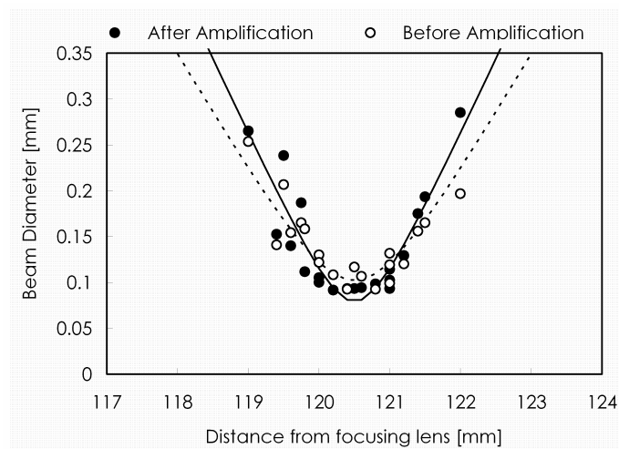
Figure.6 Dependence of focused beam diameter on the distance from the focusing lens
