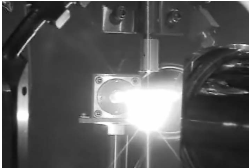
Figure.7 Xenon plasma by 1 kW (repetition rate: 100 kHz, pulse width in FWHM: 15 ns) CO 2 laser irradiation
