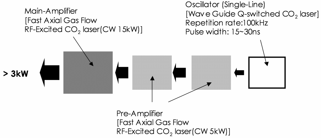
Figure.1 Configuration of the laser driver for the Xenon droplet target LPP EUV light source
