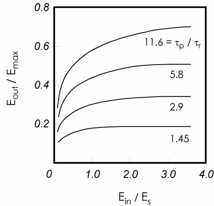
Figure.2 Calculated power extraction vs. pulse energy relations plotted for different values of the \tau_p/\tau_r parameter ( \tau_p = 1 ns, P(20) ) 16) .
