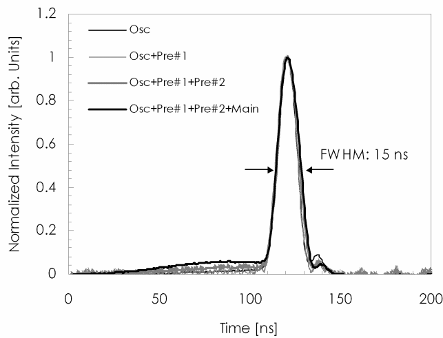
Figure.4 Input pulse of the EO Q-switched CO 2 oscillator and amplified laser pulses after each stage
