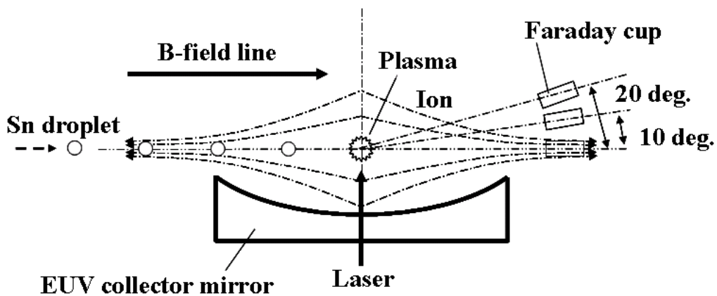
Figure 10. Experimental setup for angle distribution of ions.
