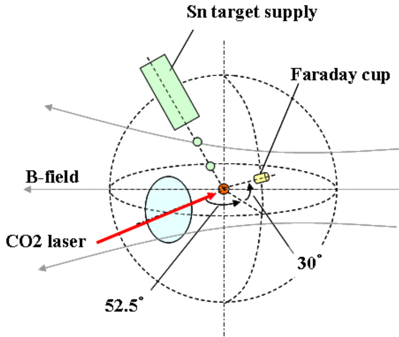
Figure 5. Experimental setup for ion mitigation measurement.
