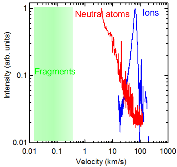
Figure 3. Velocity distribution of ions, neutrals and fragments.
