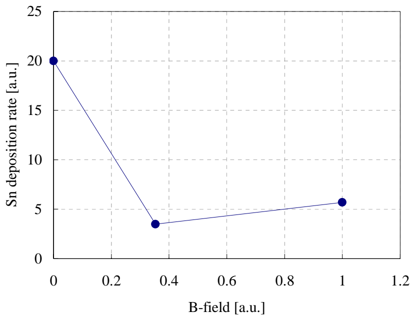
Figure 8. Dependence of Sn deposition rate on magnetic field intensity.
