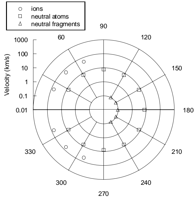
Figure 4. Peak velocity angular distribution of ions, neutrals and fragments.
