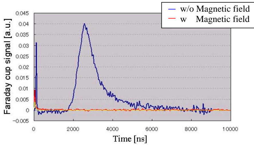
Figure 6. Faraday cup signal with and without magnetic field.
