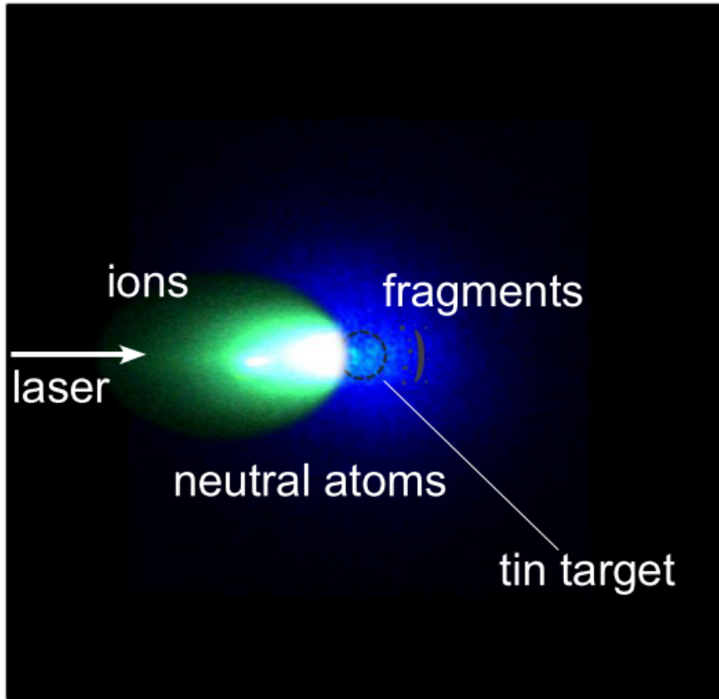
Figure 2. Schematic of the materials from the laser produced plasma with Sn droplet target.
