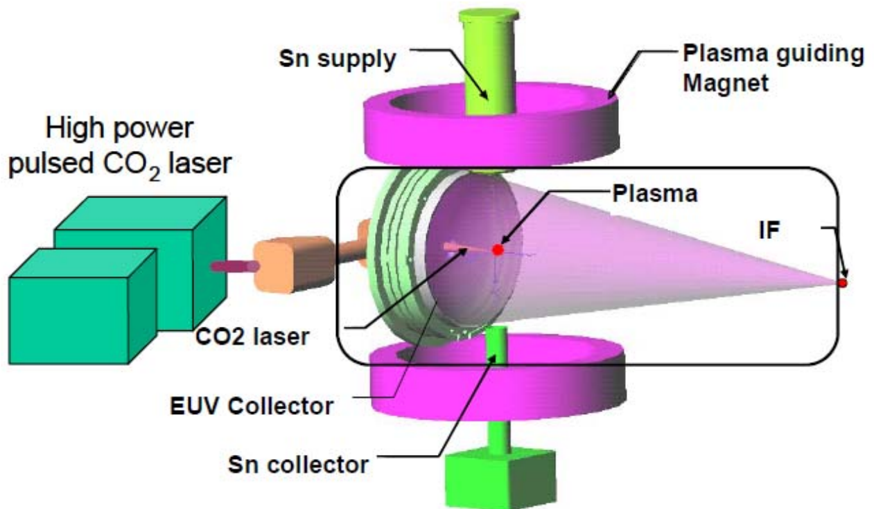
Figure 1. Concept of Laser-produced plasma light source and Magnetic field ion guiding.
