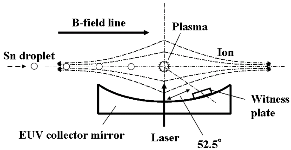
Figure 7. Experimental setup of dependence of magnetic field intensity.
