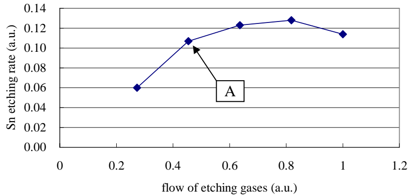
Figure 9. Dependence of Sn etching rate on etching gas flow
