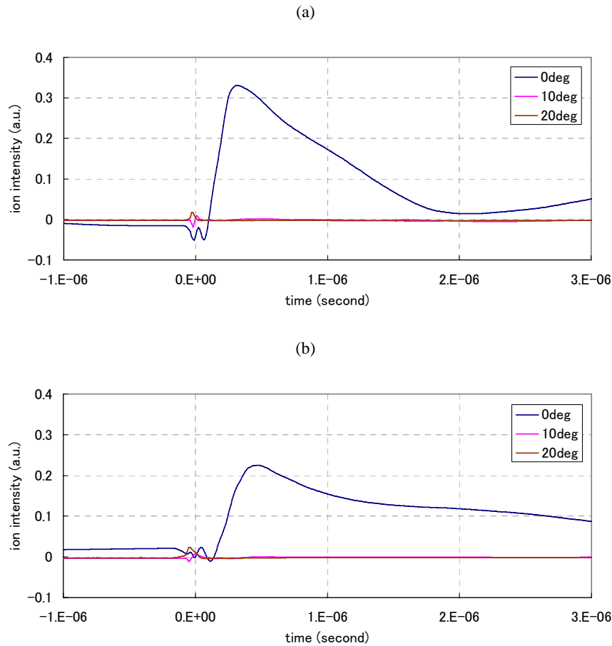
Figure 11. Faraday cup signal (a) without and (b) with etching gases
