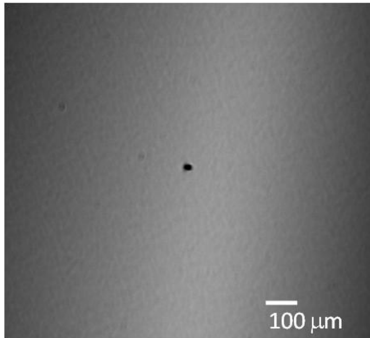
Figure 5. Shadowgraph image of 20 \mu\text{m} diameter Sn droplet
