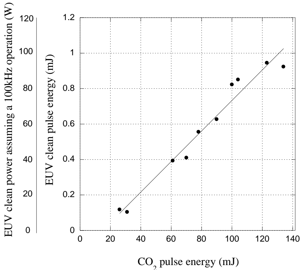
Figure 11. CO 2 pulse energy vs., EUV clean pulse energy
