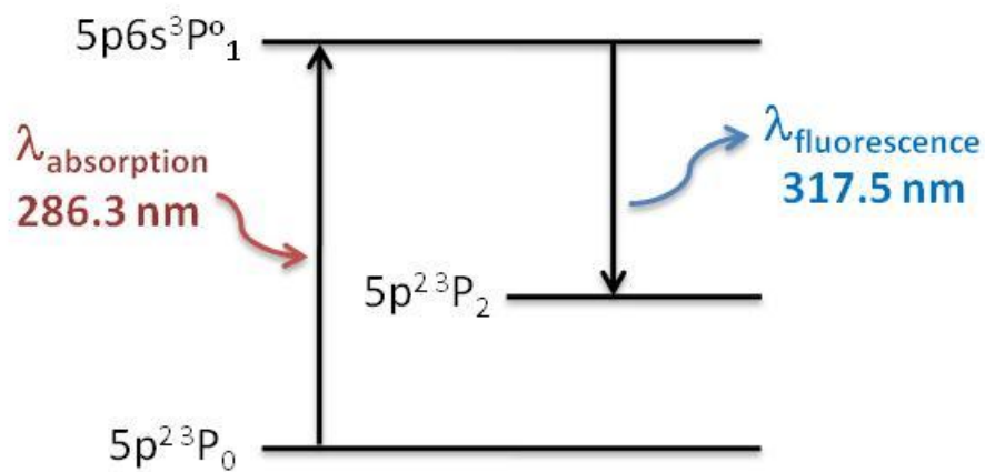
Figure 6. Energy level of Sn atom
