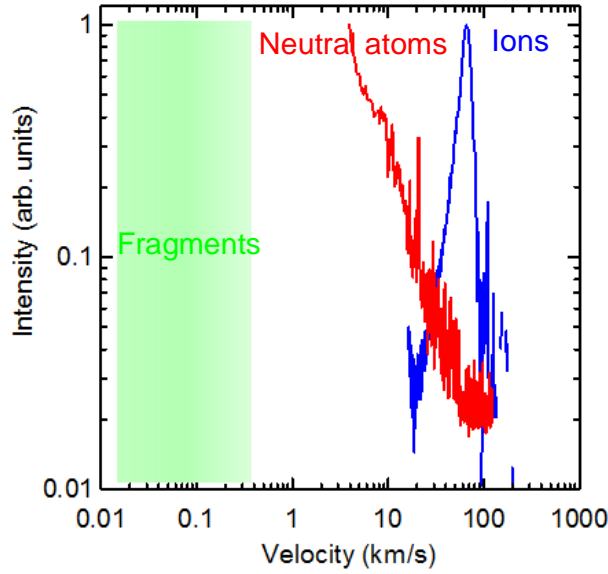
Figure 2. Velocity distribution of the Sn particles from a laser produced plasma
