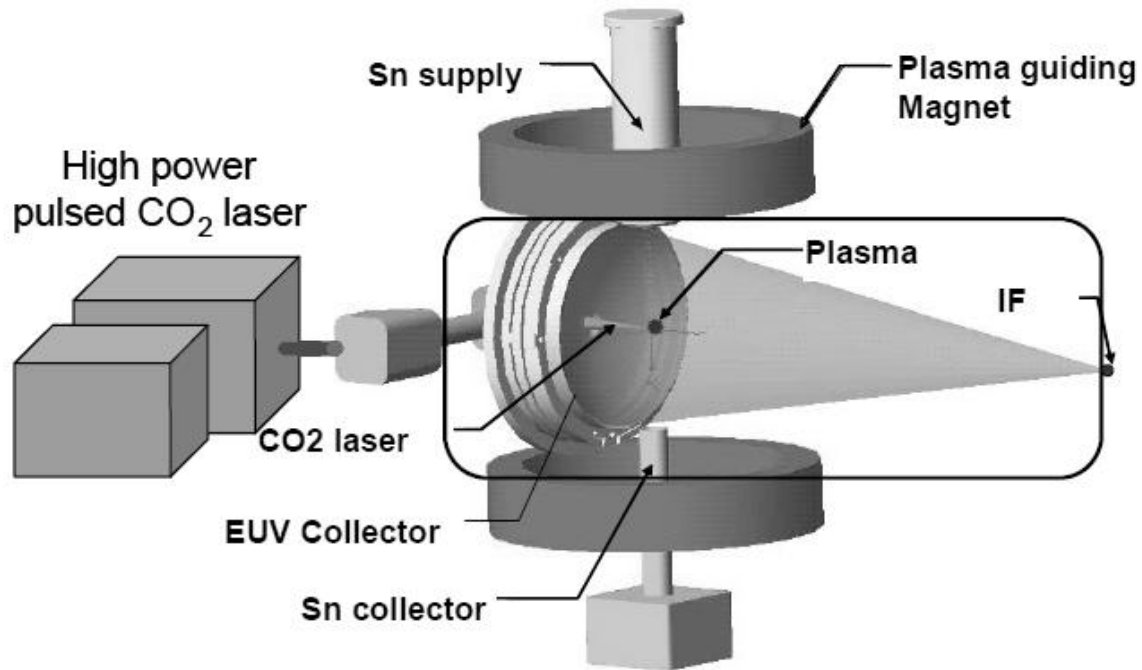
Figure 1. Schematic diagram of the developing LPP EUV light source system
