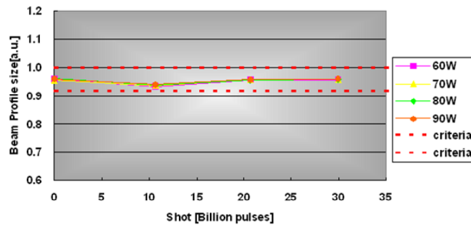
Fig.7 Output power dependency of beam profile size
