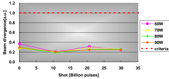
Fig.8 Output power dependency of beam divergence
