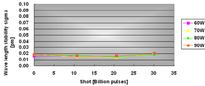
Fig.6 . Wavelength stability error from 60 to 90W
