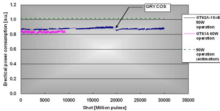
Fig.10 Electric power consumption under 90W operation to 60W
