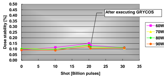
Fig.4. Dose stability trend from 60W to 90W
