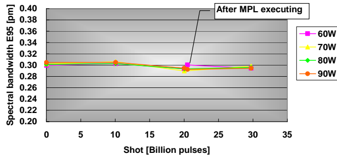
Fig.5. Spectral bandwidth from 60 to 90W
