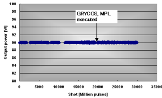
Fig.2. Pulse energy trend
