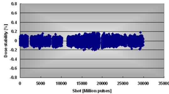
Fig.3 Dose stability trend in the durability test
